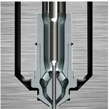
Accu-Valve GX
