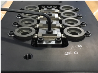
STEP 4 Re-assemble
