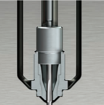
ACCU-VALVE MX (Enhanced fill balance)
