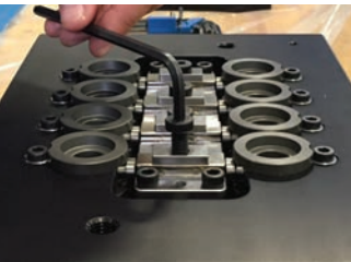
STEP 1 Remove bolt & rectangular washer
