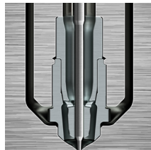
Accu-Valve CX
